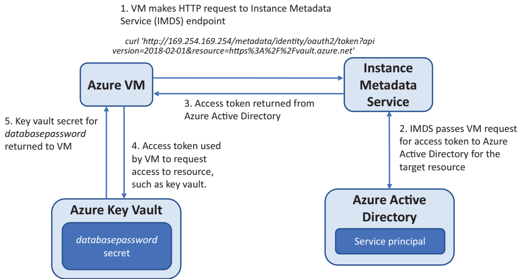
Figure 15.5 The VM uses the IMDS to request access to a key vault. The endpoint communicates with AAD to request an access token. The access token is returned to the VM, which is then used to request access from the key vault. If access is granted by the key vault, the secret for databasepassword is returned to the VM.
